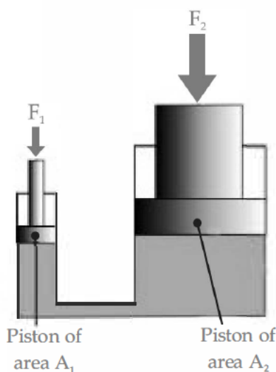
Fig 5.11 A Hydraulic machine
