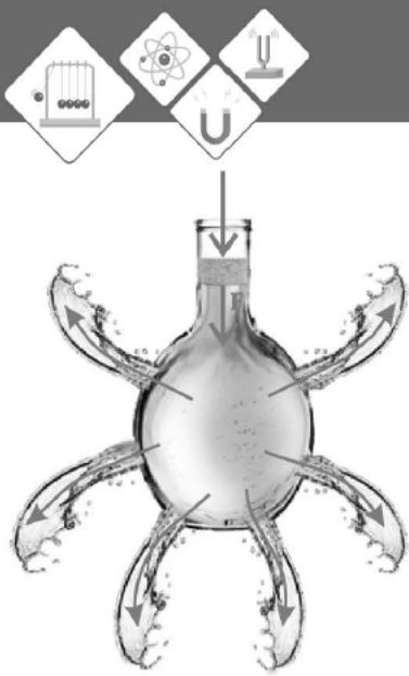
Fig 5.10 Demonstrating Pascal's law
